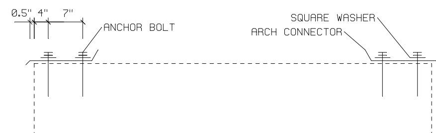
FOUNDATION END VIEW FOUNDATION WIDTH = ARCH WIDTH + 4.5"
