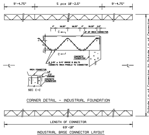
INDUSTRIAL BASE CONNECTOR LAYOUT
